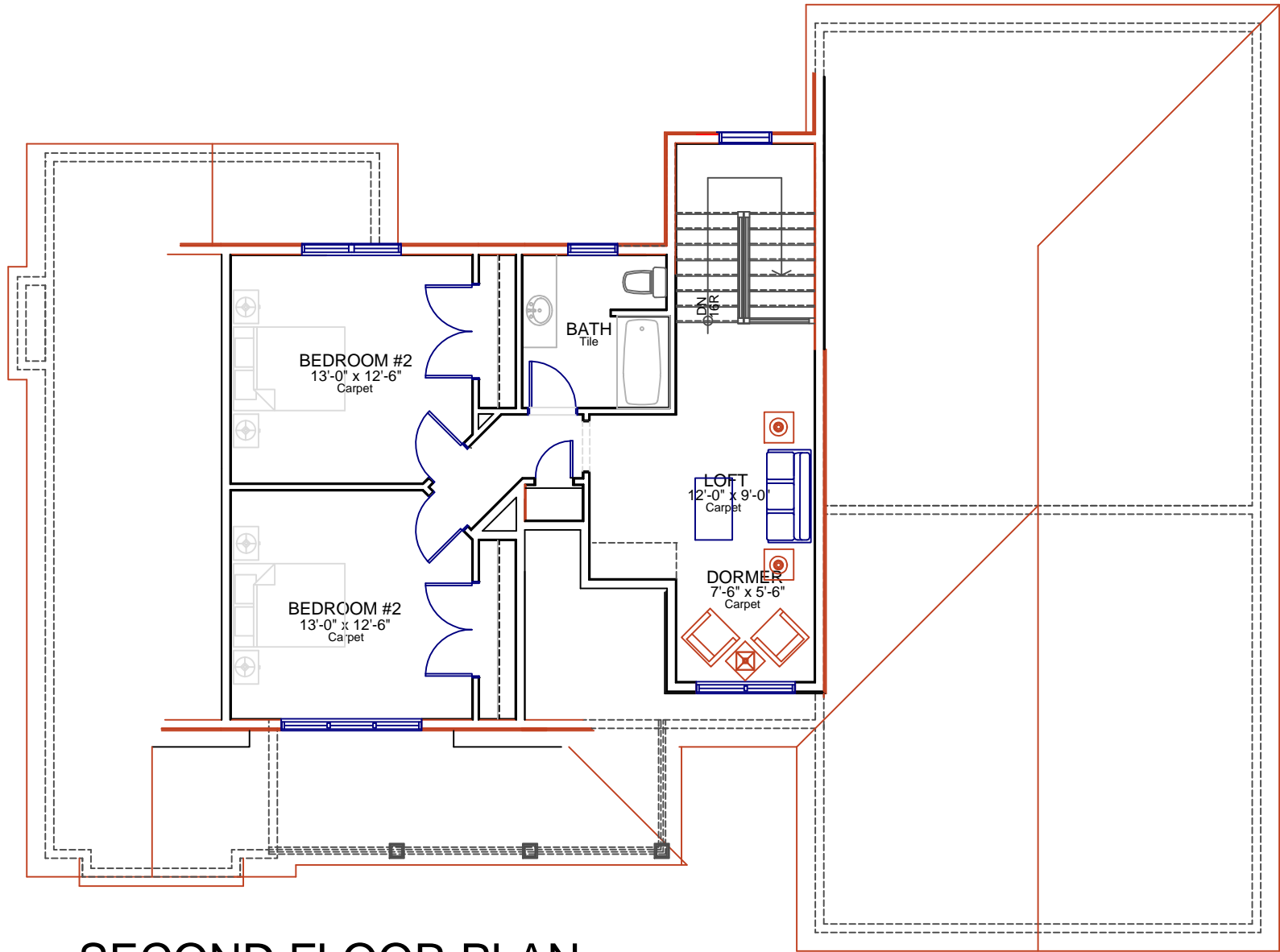
SECOND FLOOR PLAN LIVING AREA: 810 S.F.
